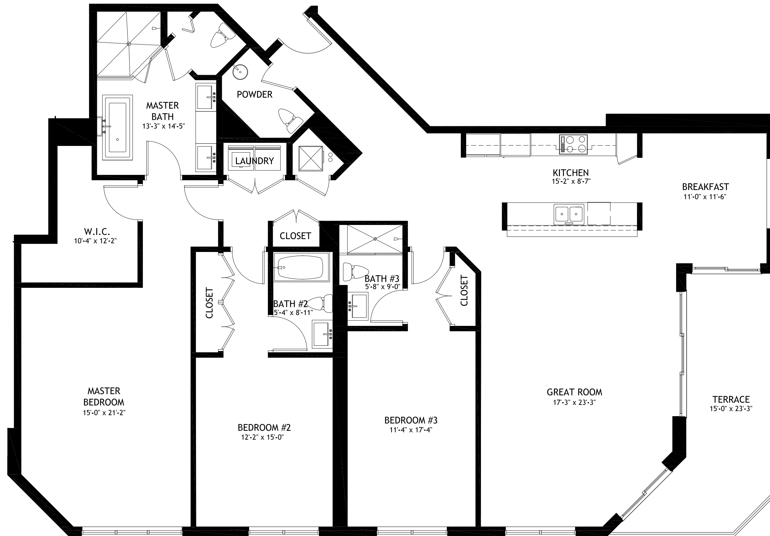
TYPICAL FLOOR
